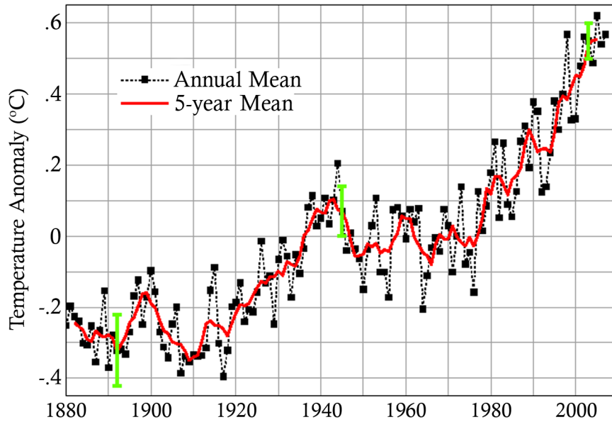
Global Temperature Land-Ocean Index
